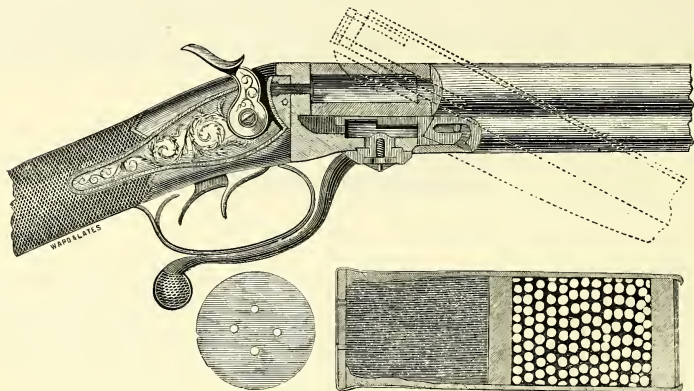
The Lancaster Central-fire Breech-loader and Cartridge.
